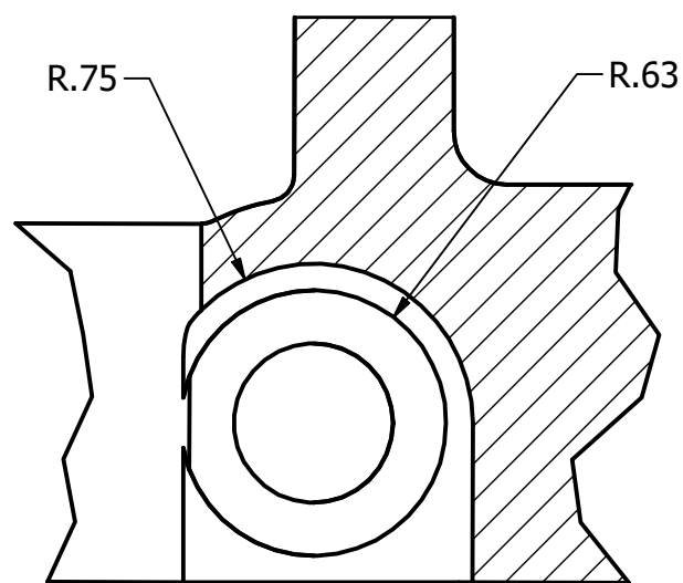
SECTION E-E SCALE 1 : 1
