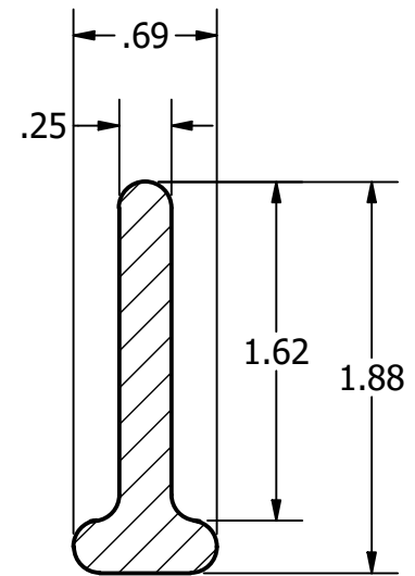
SECTION B-B SCALE 1 : 1
