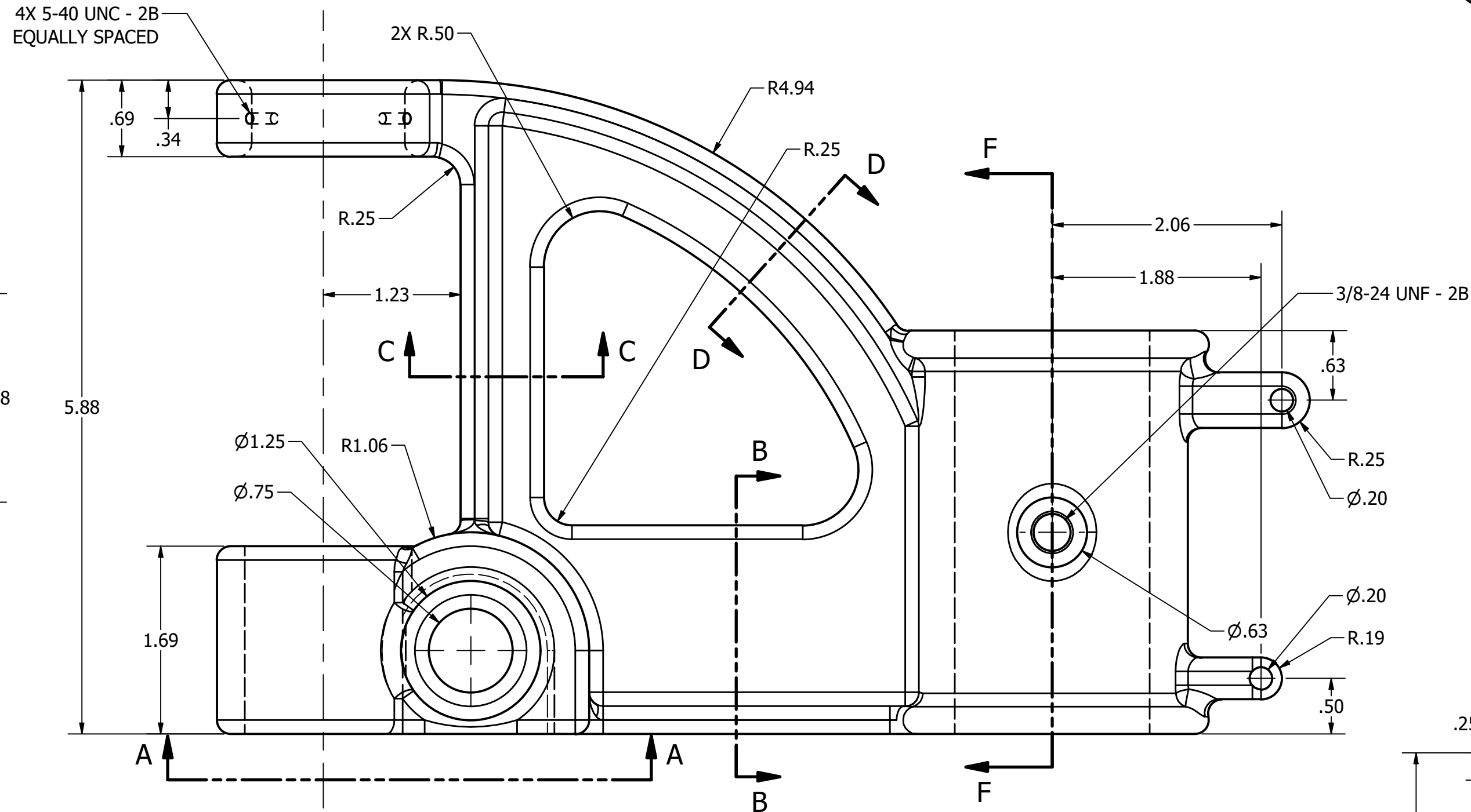
DRILL PRESS BRACKET SCALE 1 : 1
