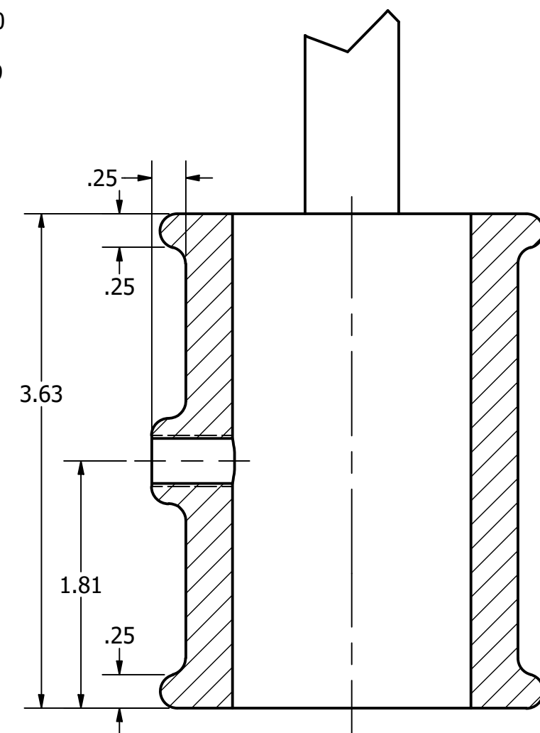
SECTION F-F SCALE 1 : 1
