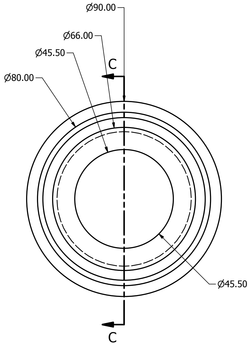
WHEEL SCALE 1 : 1
