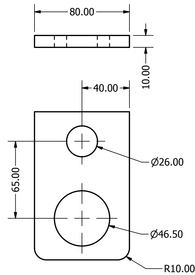
SMALL PLATE SCALE 1 / 2
