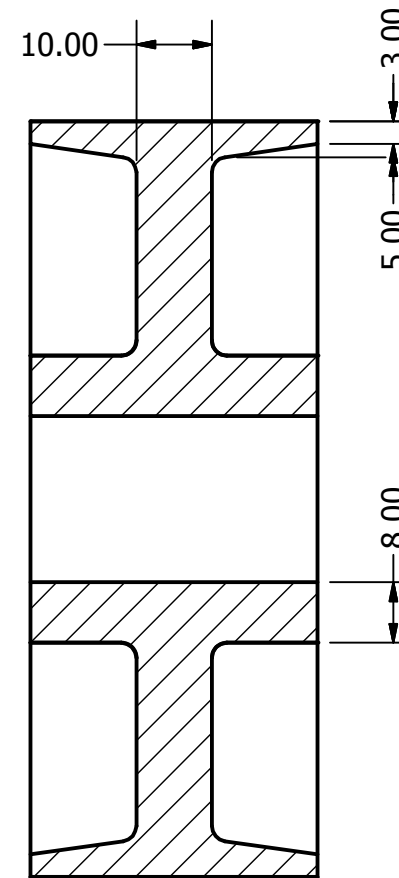
SECTION B-B SCALE 1 : 1
