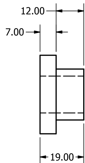
BUSHING SCALE 1 : 1
