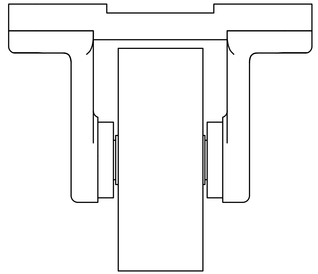
CASTER ASSEMBLY SCALE 1 : 1
