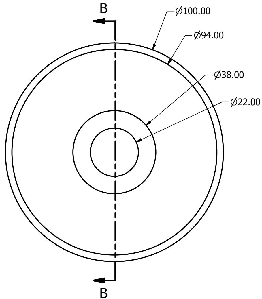
WHEEL SCALE 1 : 1
