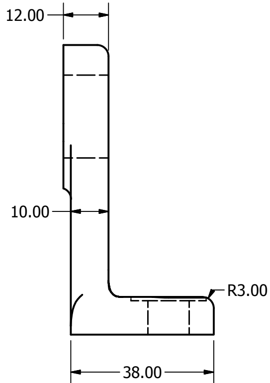
AXLE SUPPORT SCALE 1 : 1
