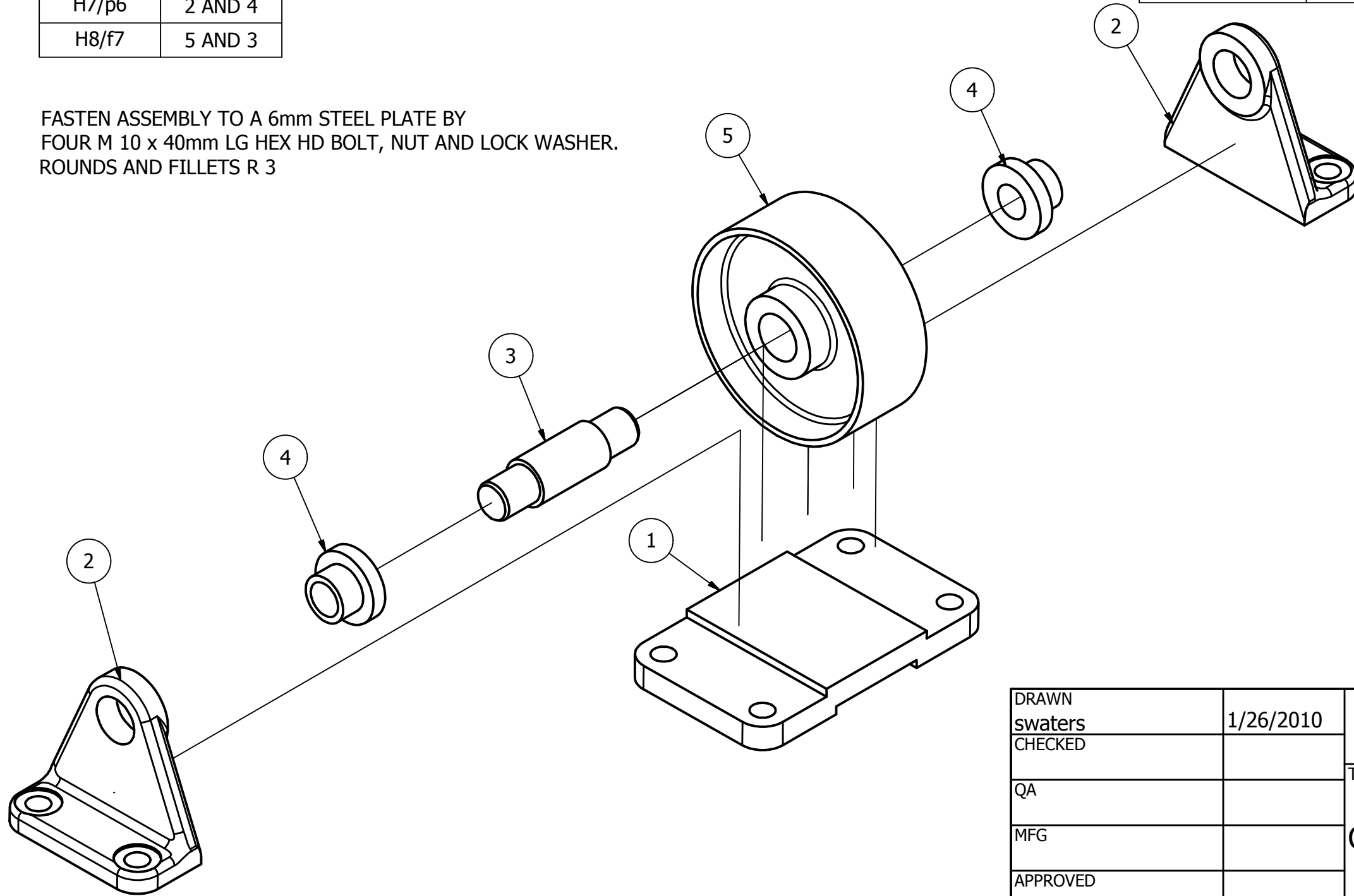
CASTER ASSEMBLY EXPLODED SCALE 1 / 2
