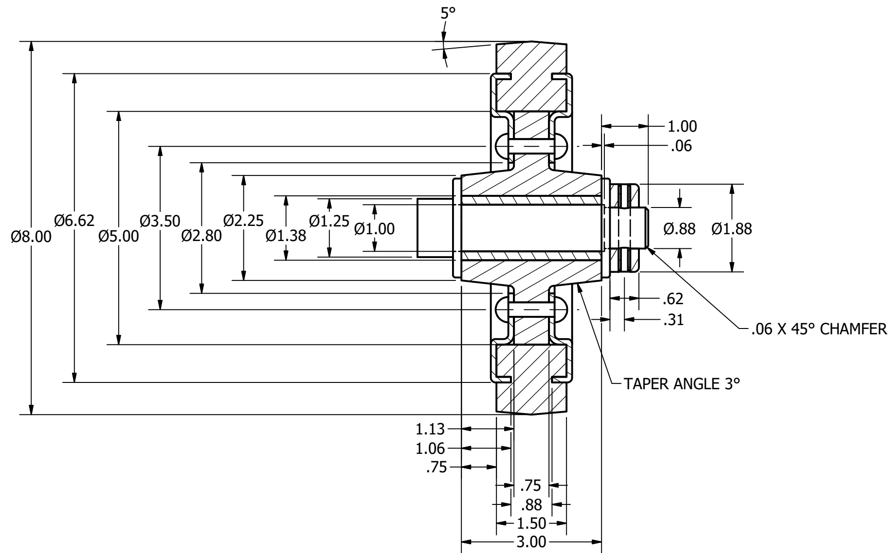
WHEEL ASSEMBLY SECTION VIEW SCALE 1 / 2
