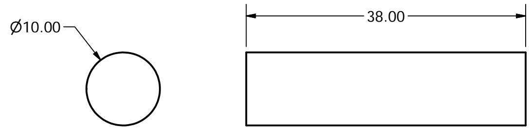
PT5 ROLLER BEARING SCALE 2 : 1
