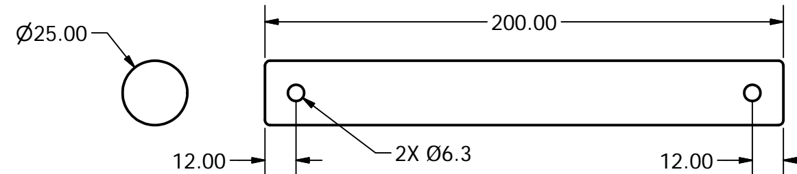
PT3 AXLE SCALE 1 / 2
