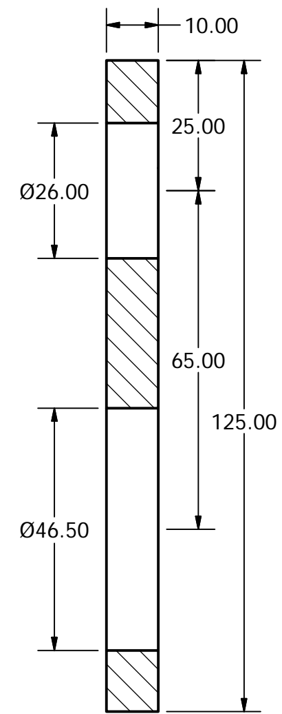
SECTION E-E SCALE 1 : 1
