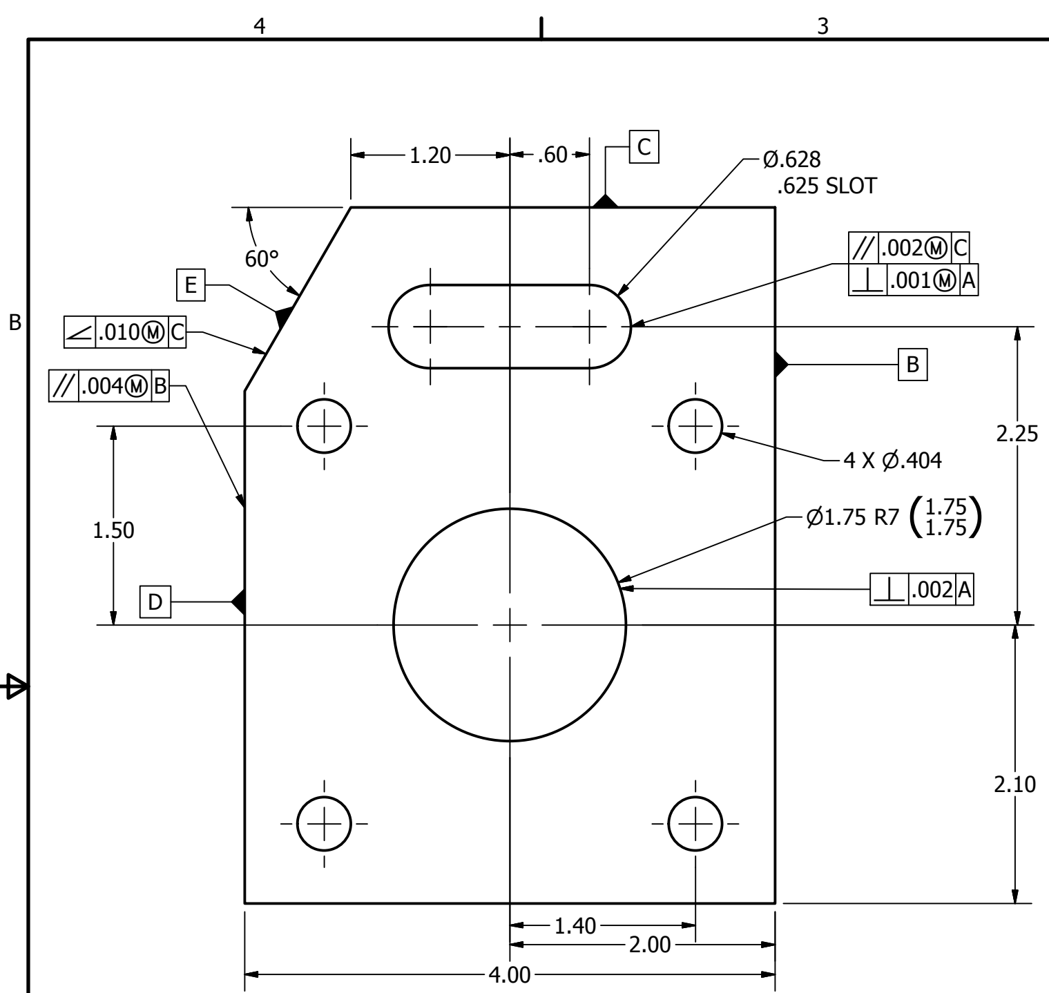
SPACER PART SCALE 1 : 1
