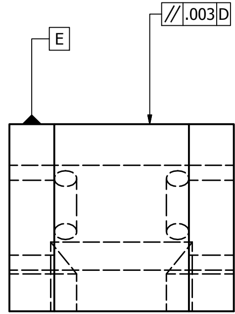
VIEW B-B SCALE 1 : 1
