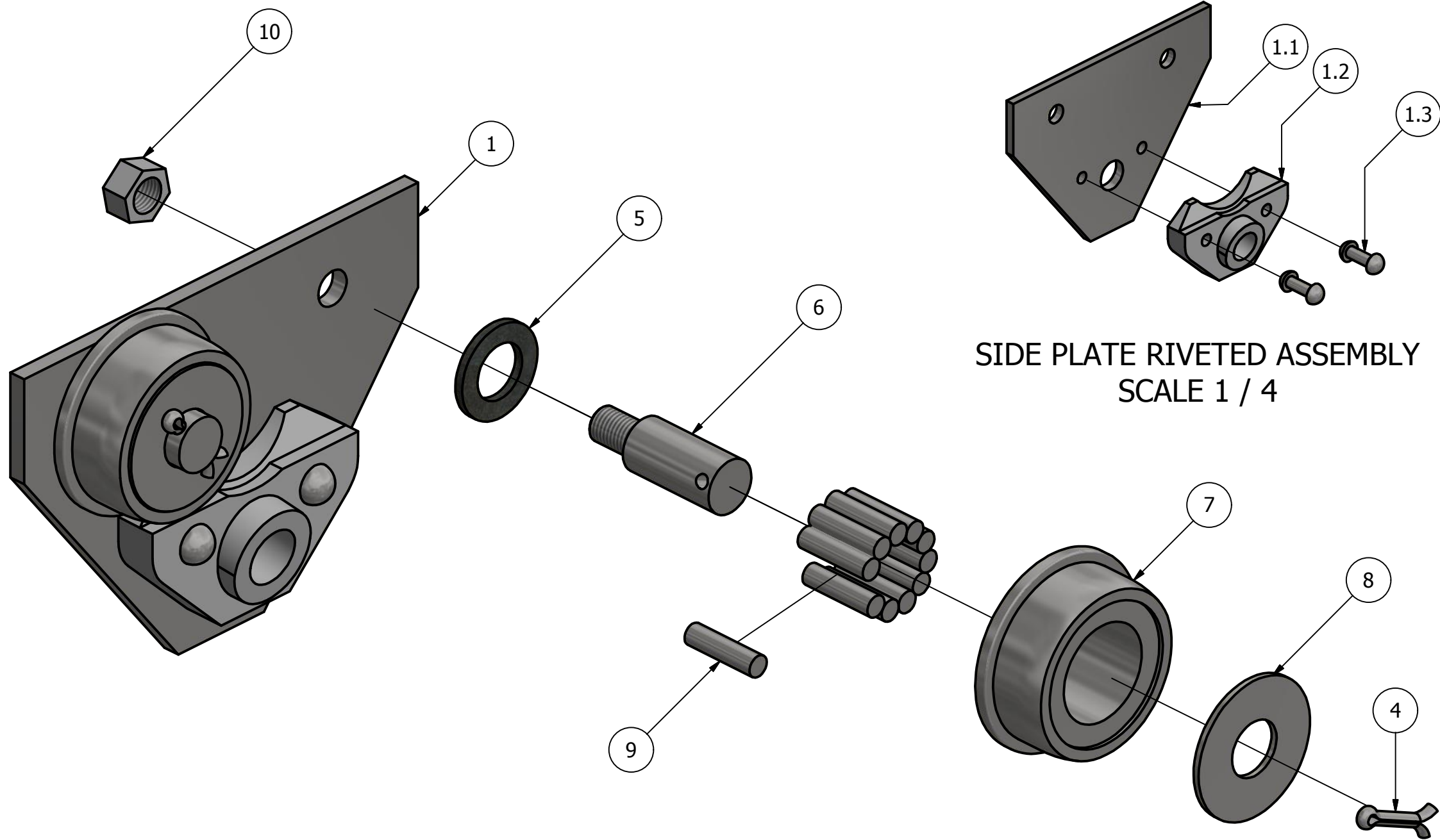
SIDE PLATE WITH WHEELS EXPLODED ASSEMBLY SCALE 1 / 2
