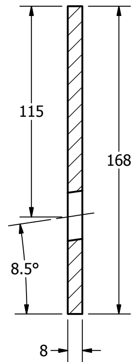
SECTION A-A SCALE 1 / 2
