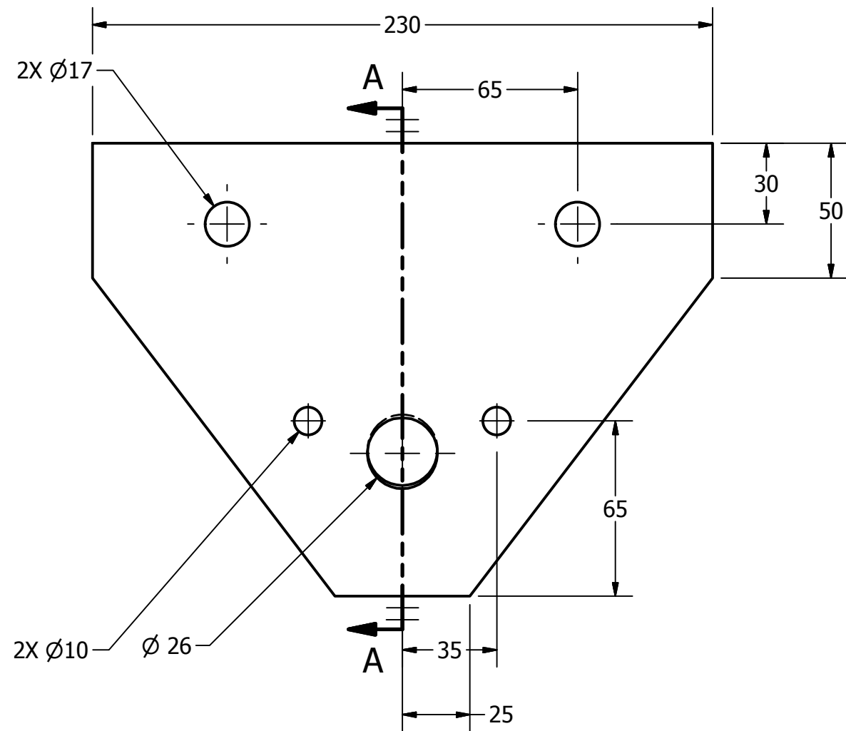
SIDE PLATE SCALE 1 / 2
