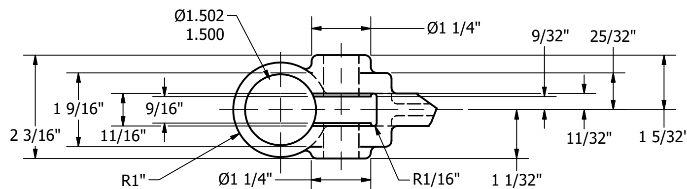
VIEW D-D SCALE 1 / 2
