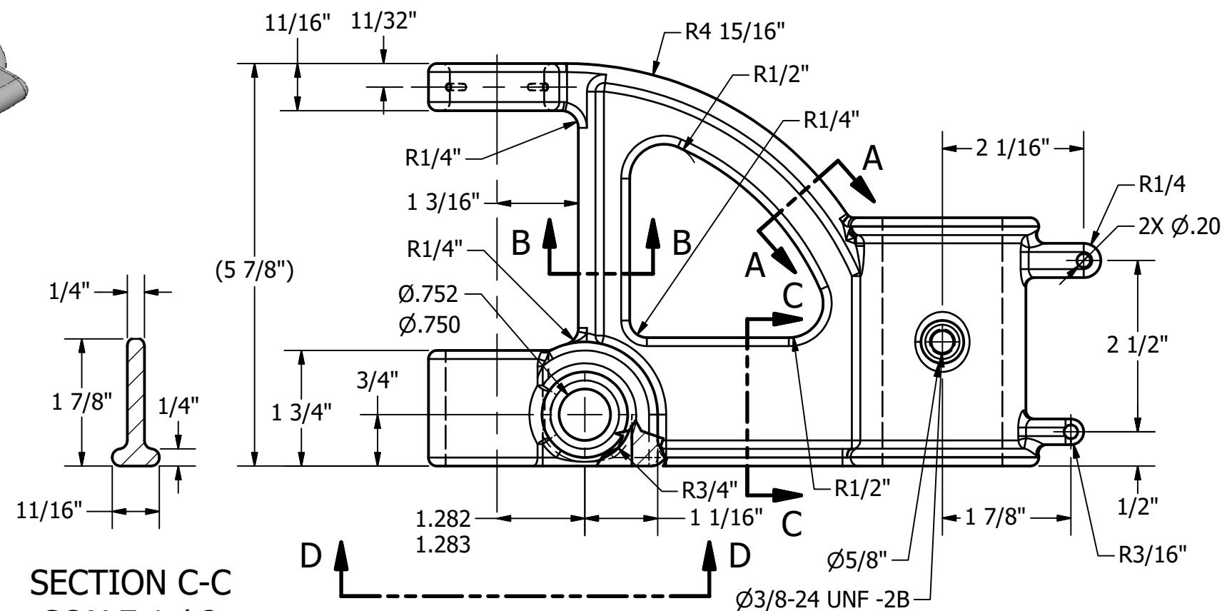
DRILL PRESS BRACKET SCALE 1/2
