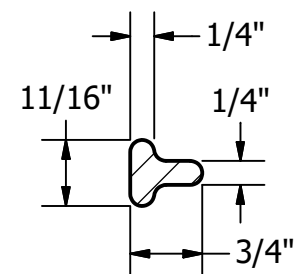
SECTION B-B SCALE 1 / 2
