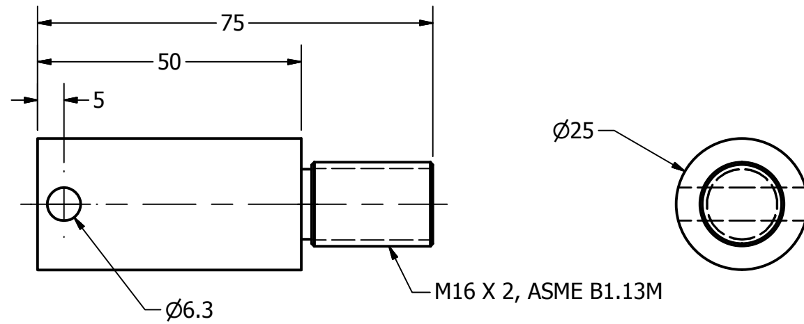
AXLE SCALE 1 : 1
