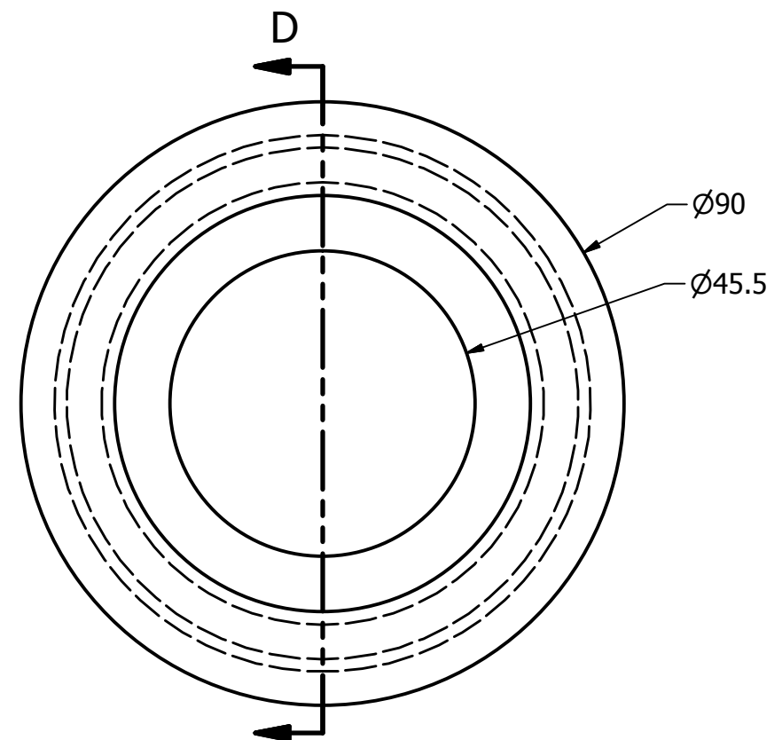
WHEEL SCALE 1 : 1
