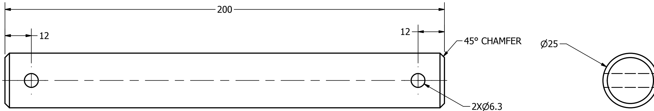
AXLE SCALE 1 : 1
