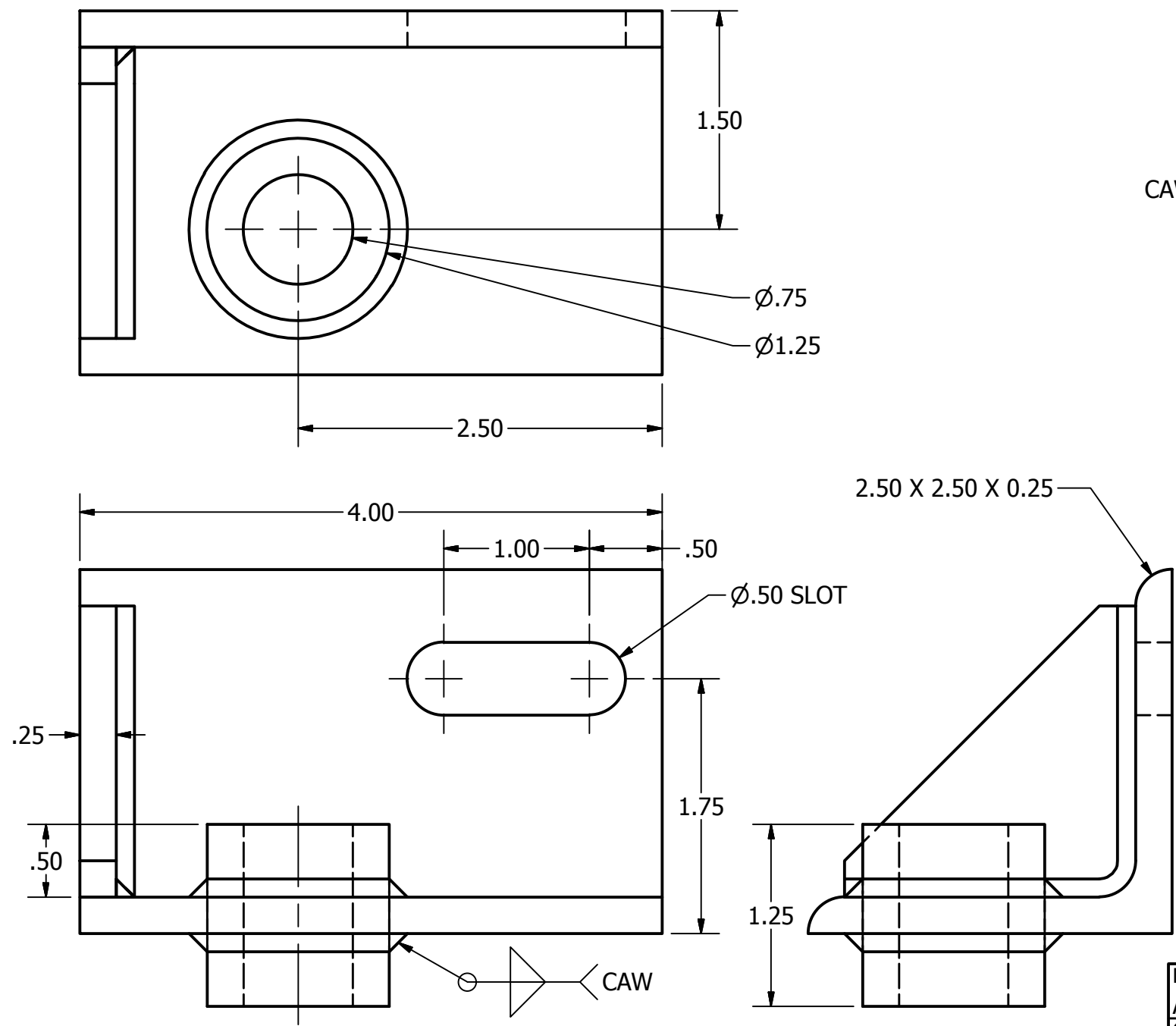
FIG 18-43 SLIDE BRACKET SCALE 1 : 1
