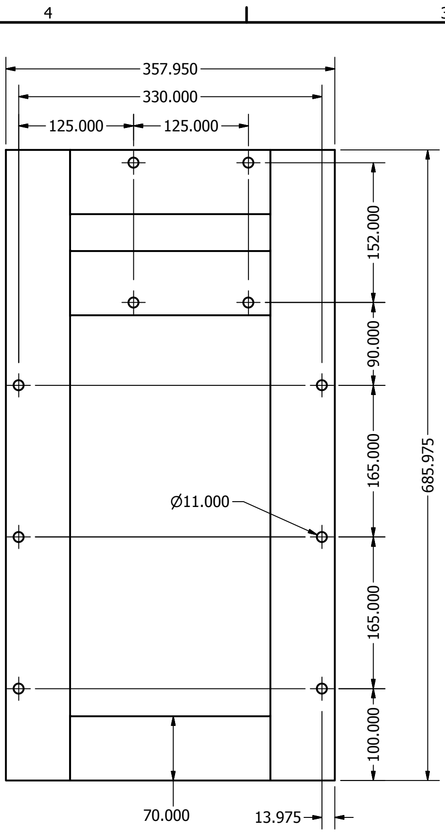
FRAME ASSEMBLY SCALE 1 / 4
