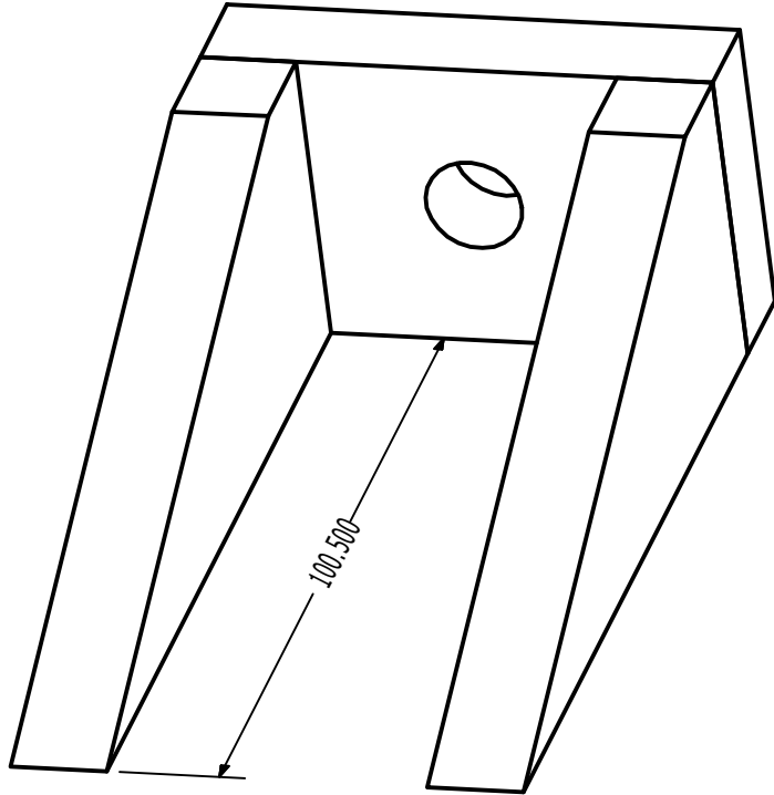
UNDER-SIDE SCALE 1 : 1
