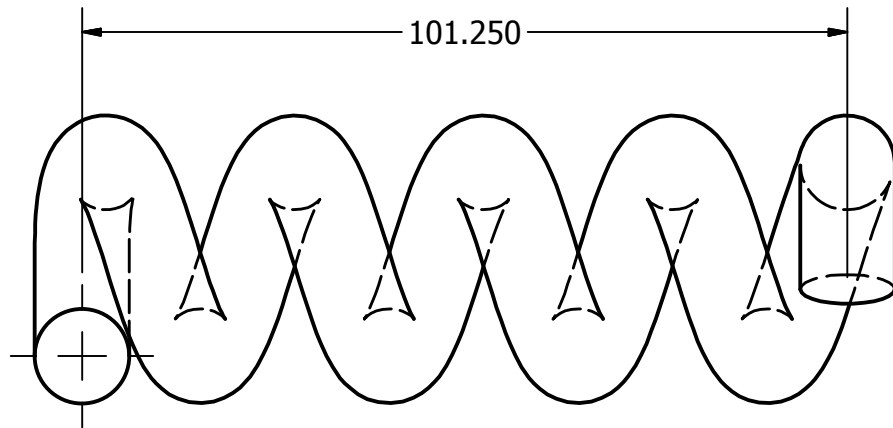
SPRING SCALE 1 : 1
