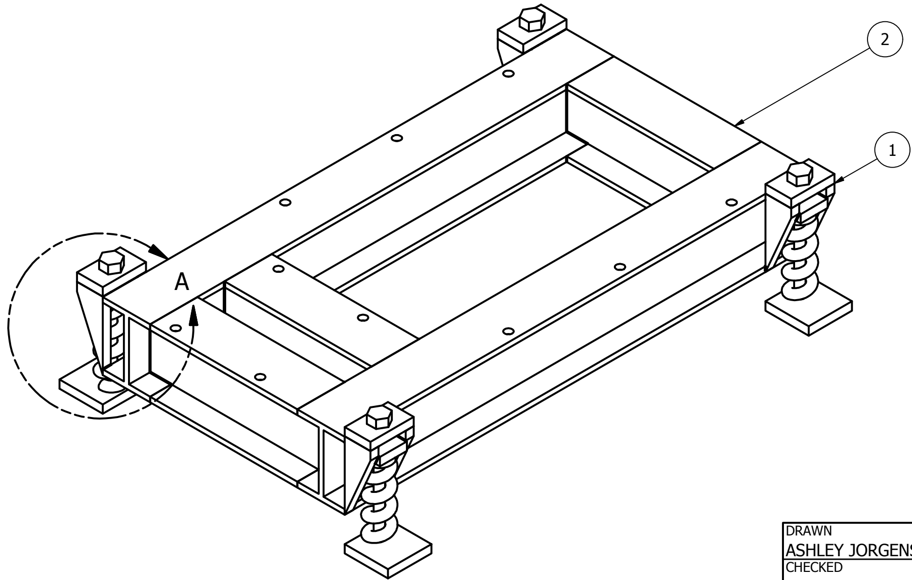
FAN AND MOTOR BASE SCALE 1 / 4
