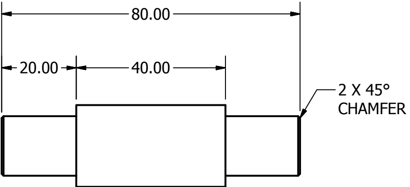
AXLE SCALE 1 : 1
