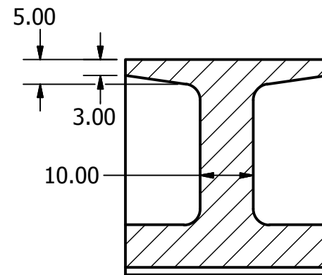
SECTION B-B SCALE 1 : 1
