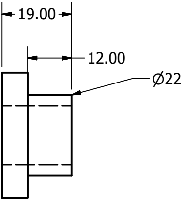
BUSHING SCALE 1 : 1
